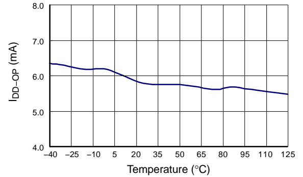
Figure 9. Operating Current
