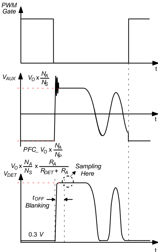
Figure 45. Operation Waveform of Output Over-Voltage Detection
