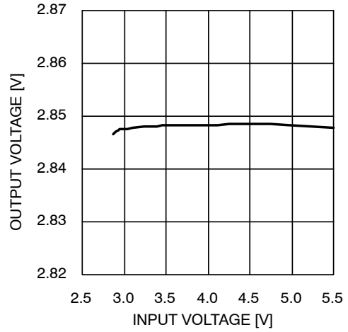
Figure 4. Line Regulation
