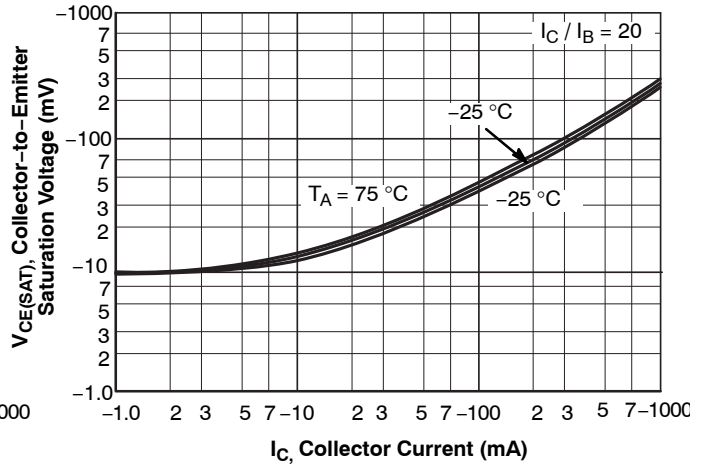
Figure 5. V_{CE(sat)} - I_C
